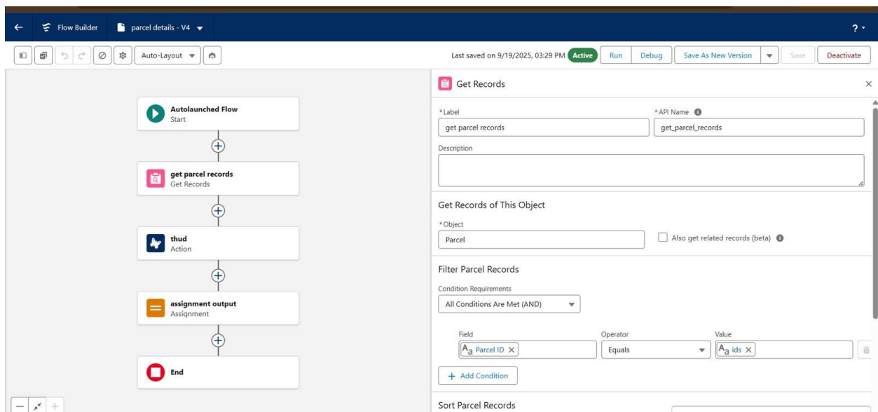
Figure 42: Get Records element – Parcel filtered by Parcel ID
