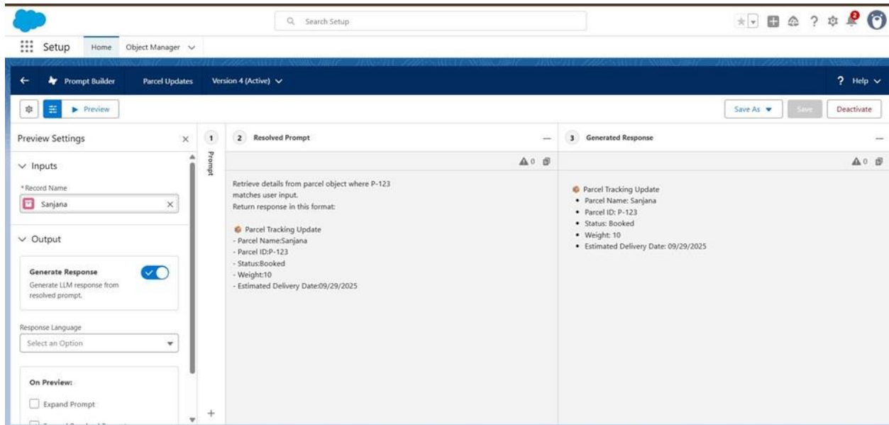
Figure 37: Prompt preview – resolved prompt and generated response
