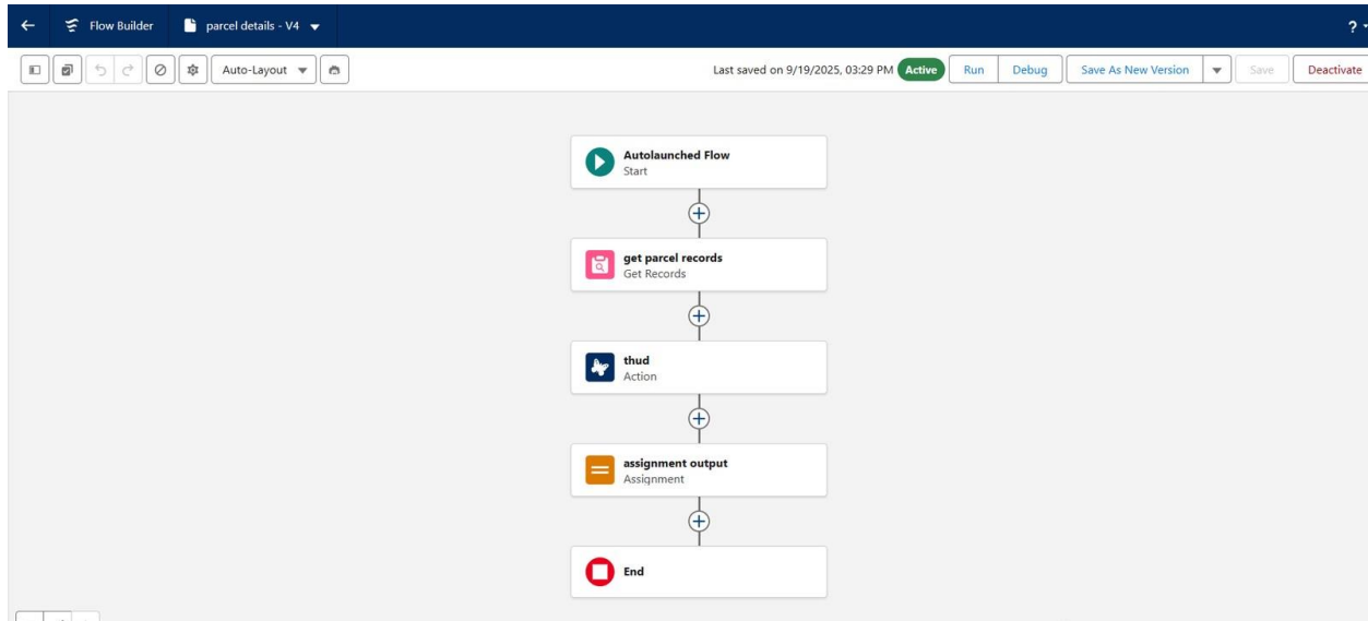
Figure 74: Parcel Details Flow – Start, Get Records, Action, Assignment, End
