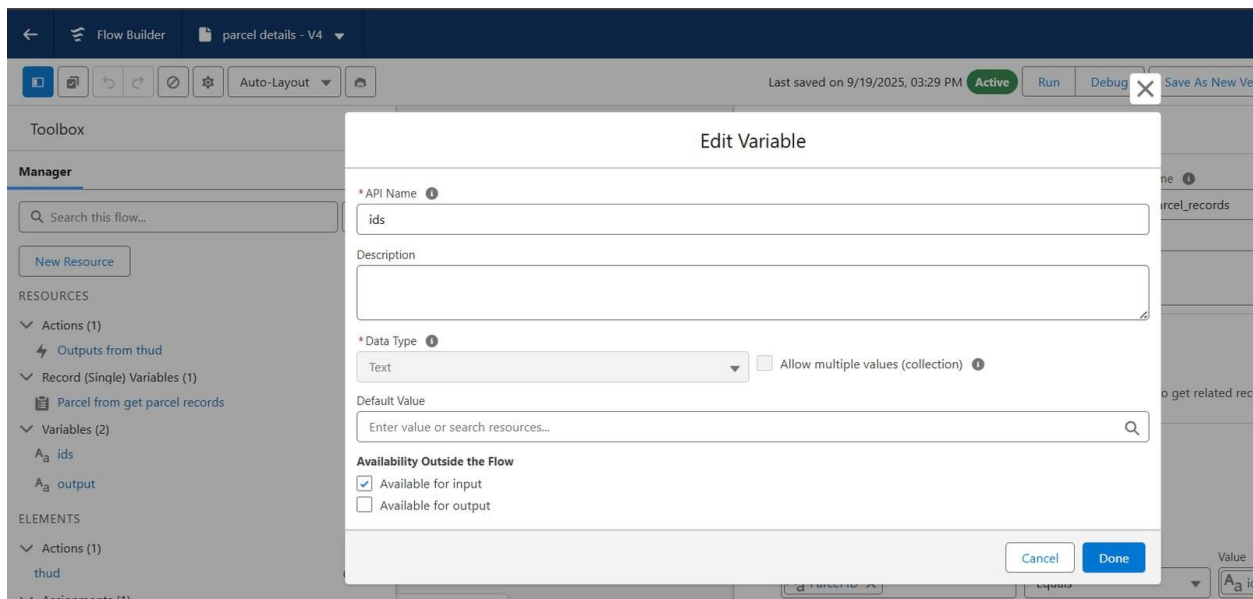
Figure 40: Edit Variable – ids (available for input)
