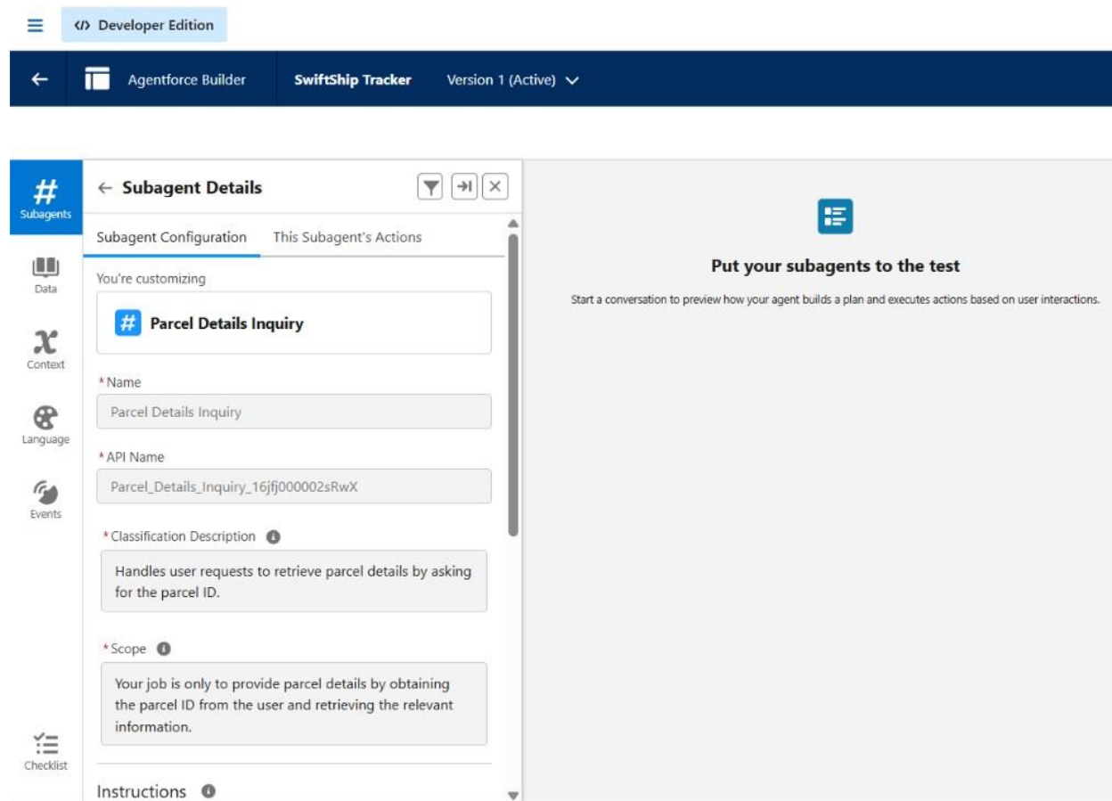
Figure 72: Subagent configuration – Parcel Details Inquiry
