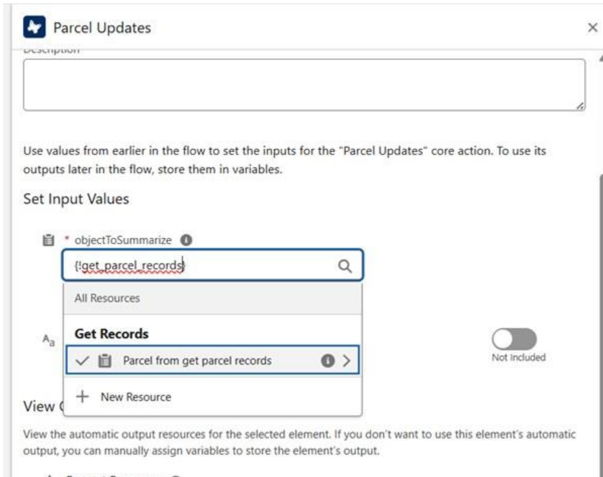
Figure 43: Parcel Updates action – Object To Summarize
