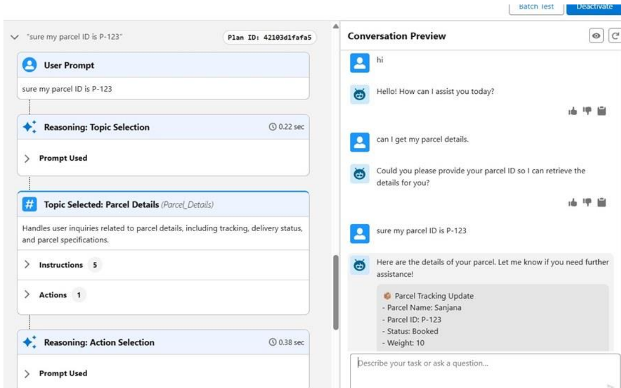
Figure 75: Agent conversation preview – parcel details returned for a Parcel ID
